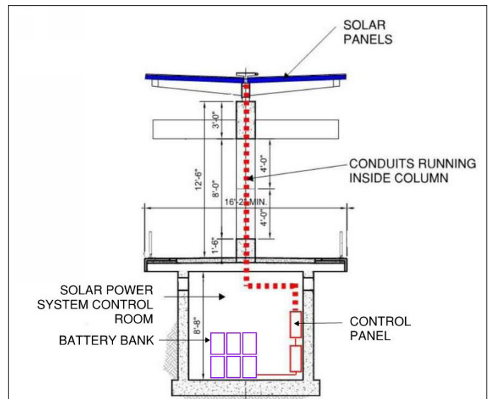
Figure 3-5 Proposed concept for a solar power system control room and battery bank below platform, at-grade stations. A similar layout should be used for aerial stations.
