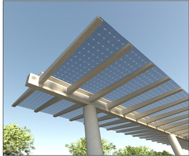
Figure 3-2 Rendered concept of continuous bifacial solar panels on Systemwide Station Design (SWSD) canopy.
