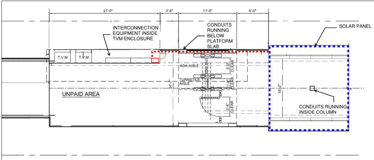
Figure 3-6 Proposed concept for a solar power system control room inside TVM chase of an at-grade station.
