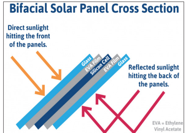
Figure 4-2 Bifacial solar panel schematic section.
